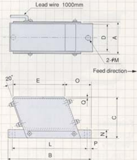
MF-04B/15B Dimensions
